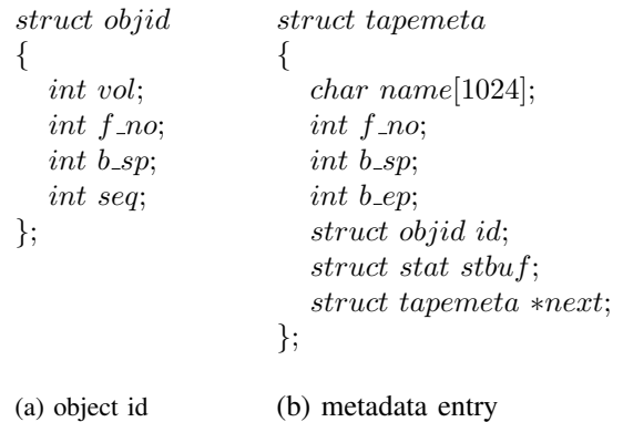
Fig. 3. Data structure
